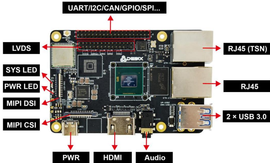
Figure 2 DEBIX Infinity Front interface
