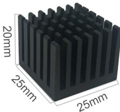
Figure 76 Aluminum alloy heatsink
