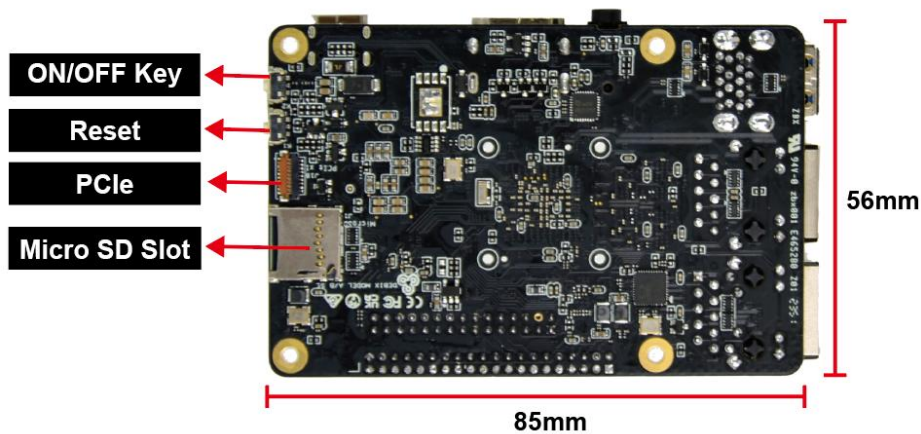
Figure 3 DEBIX Infinity Back interface
