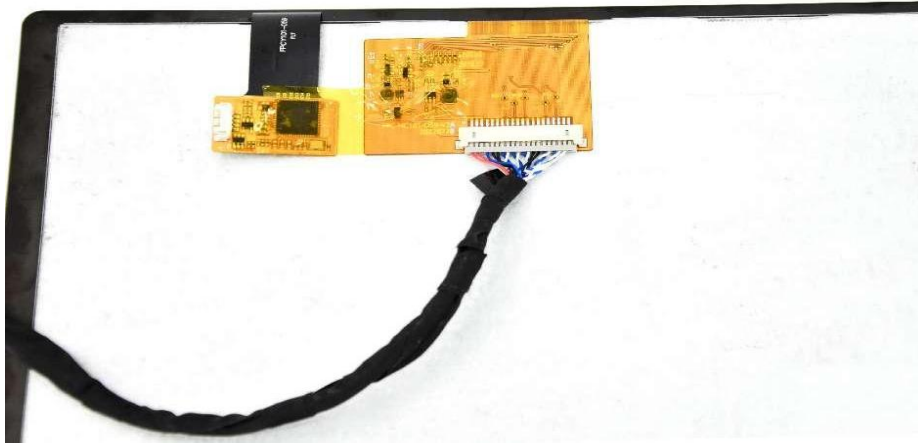
Figure 65 Connect LVDS screen cable to LVDS screen
